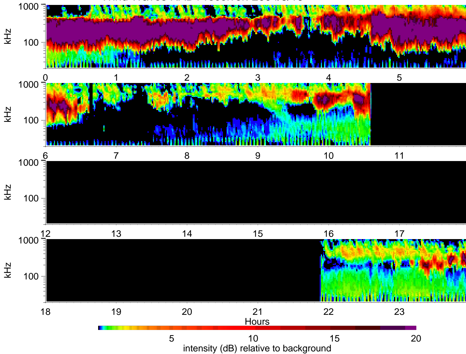
Wind Waves RAD1 receiver: 2004/3/19
