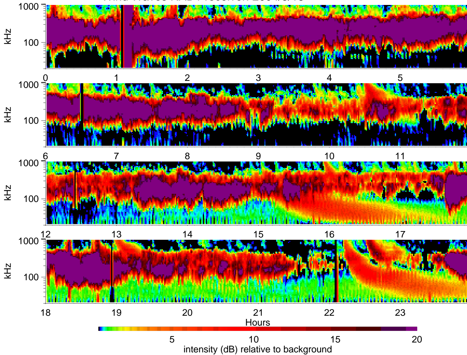
Wind Waves RAD1 receiver: 2004/3/18
