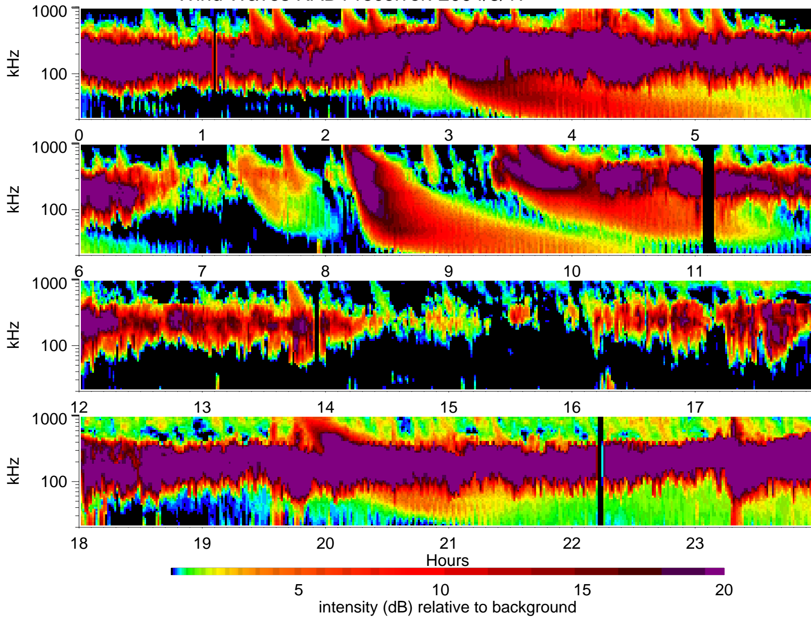
Wind Waves RAD1 receiver: 2004/3/17
