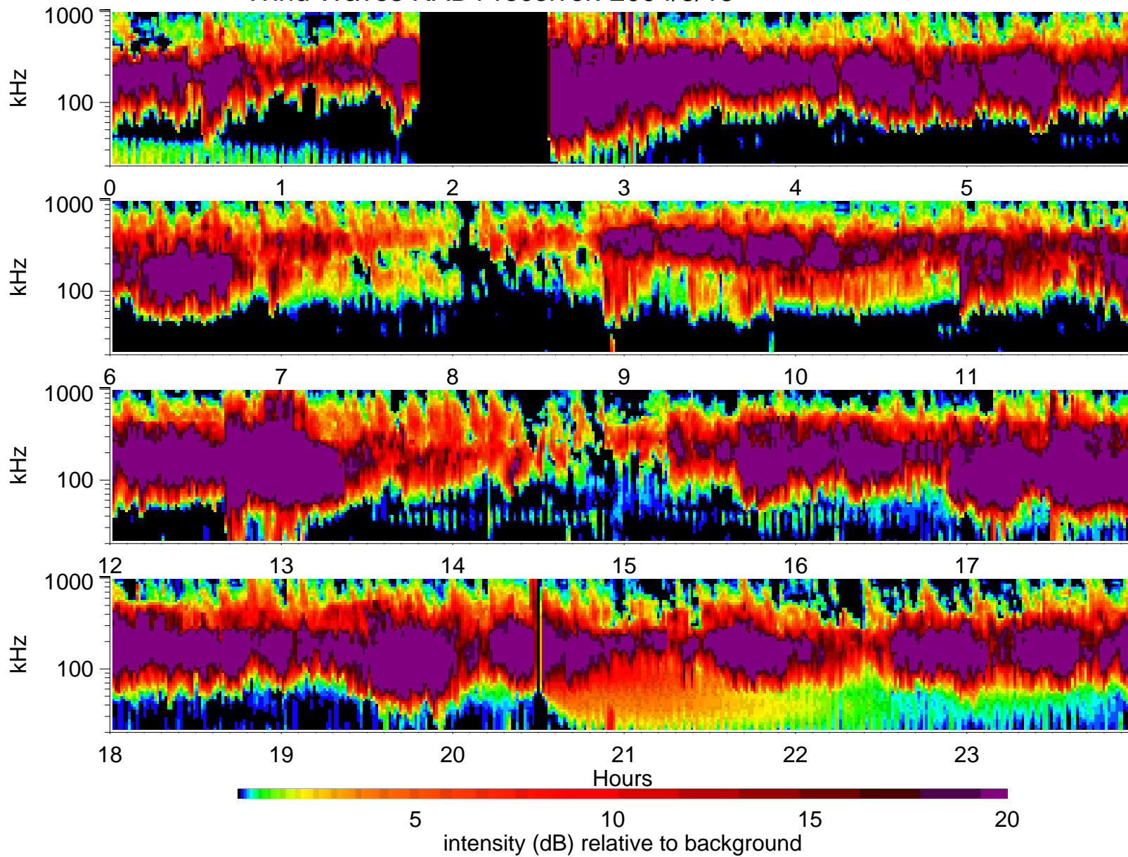
Wind Waves RAD1 receiver: 2004/3/15
