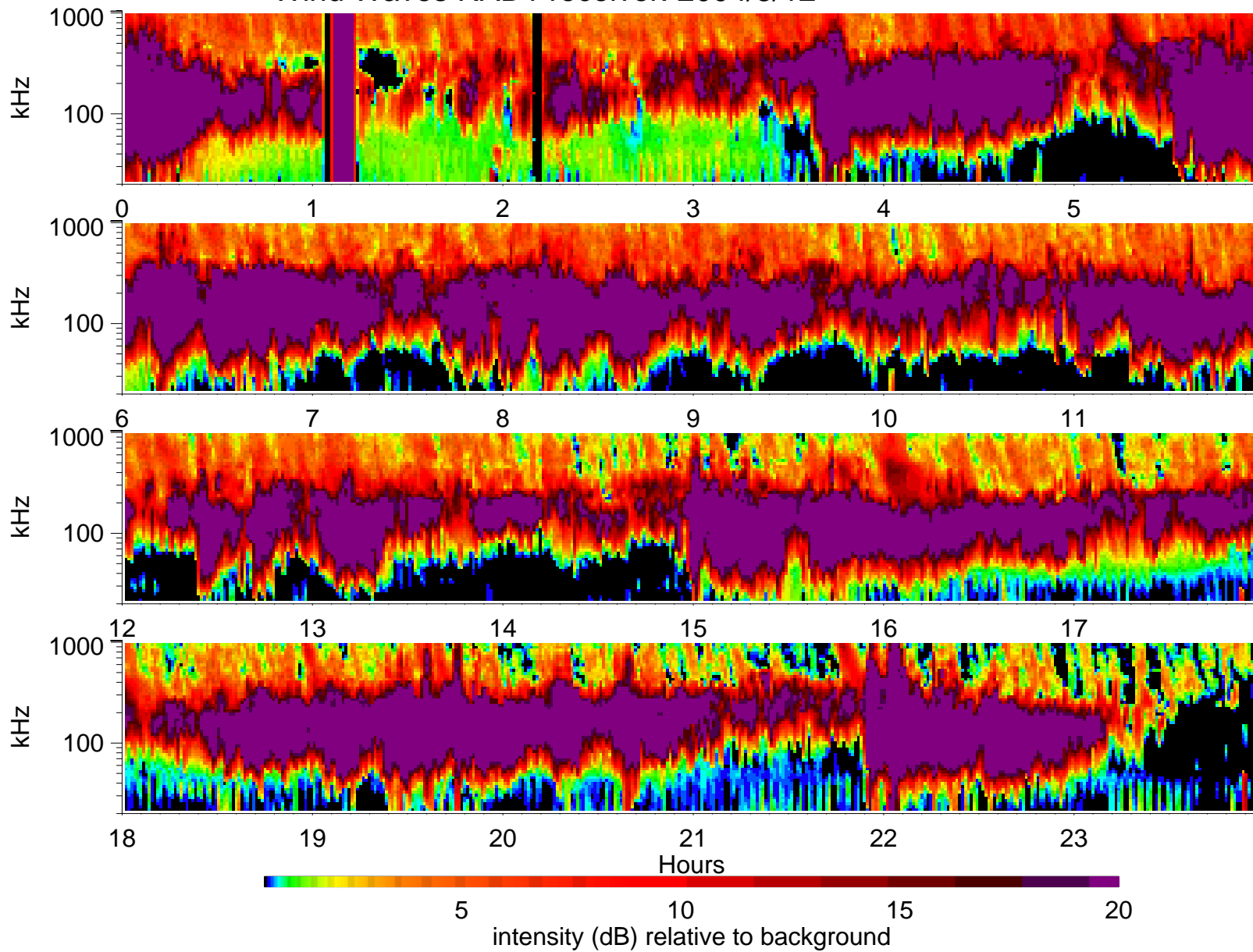
Wind Waves RAD1 receiver: 2004/3/12
