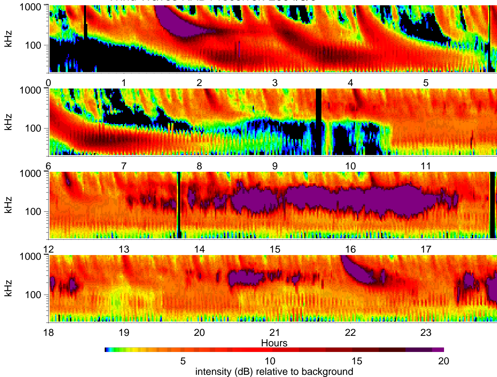
Wind Waves RAD1 receiver: 2004/3/9
