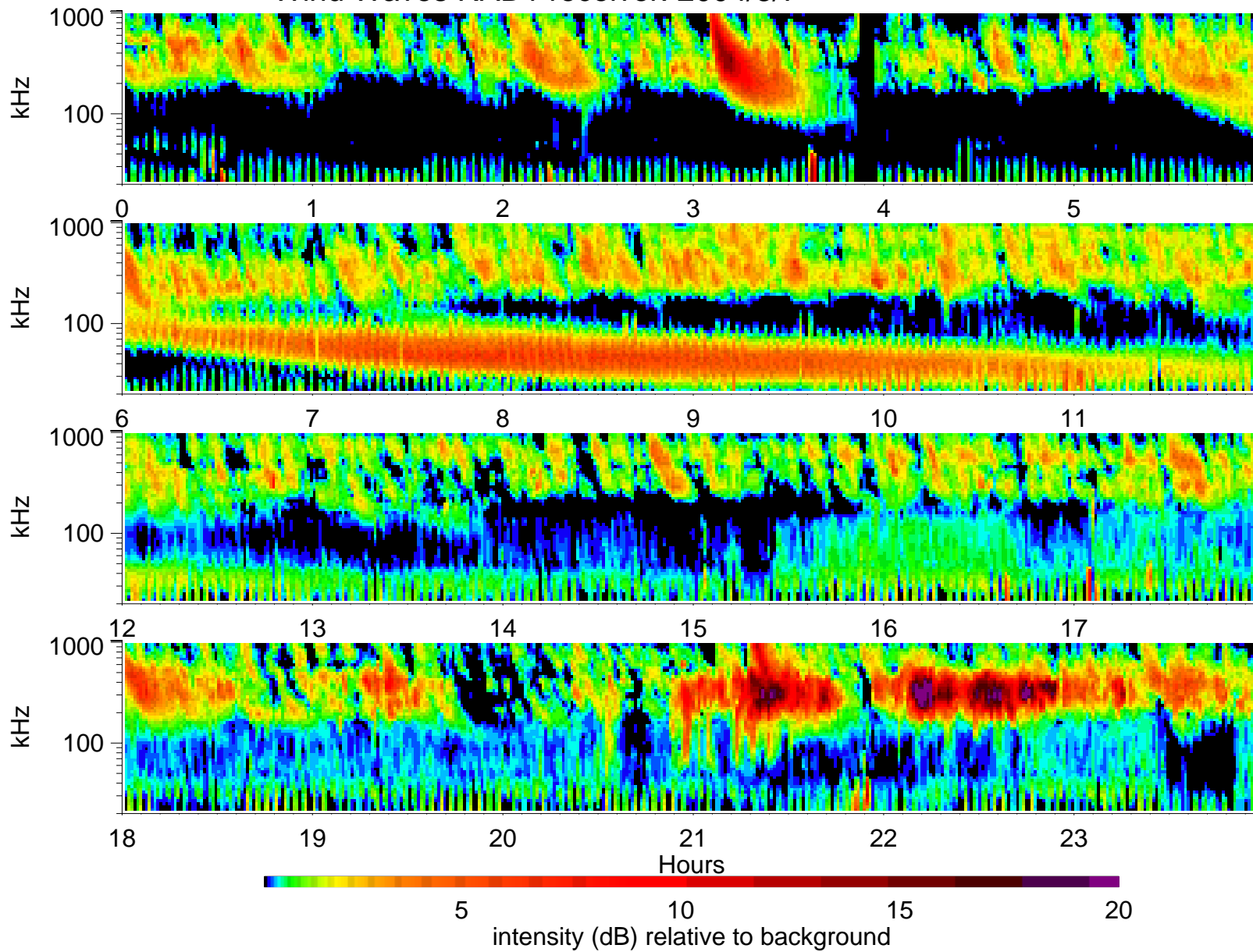
Wind Waves RAD1 receiver: 2004/3/7
