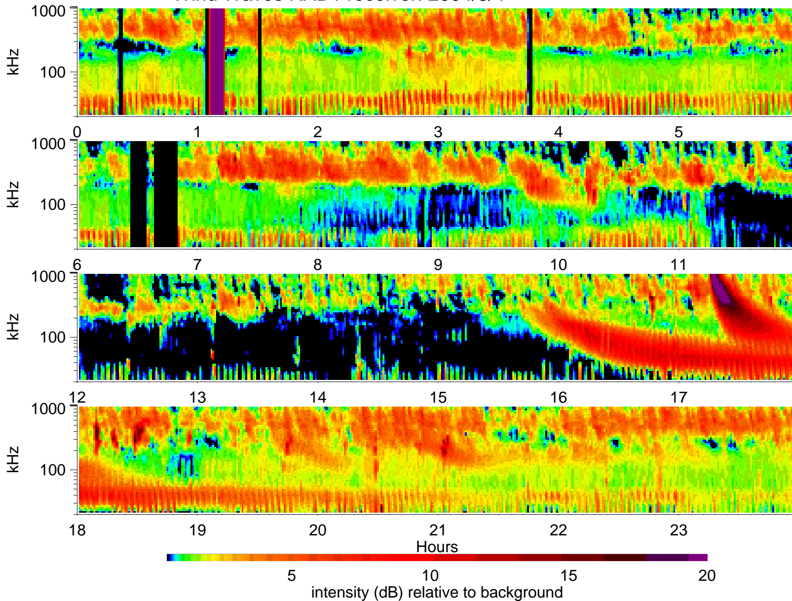
Wind Waves RAD1 receiver: 2004/3/4
