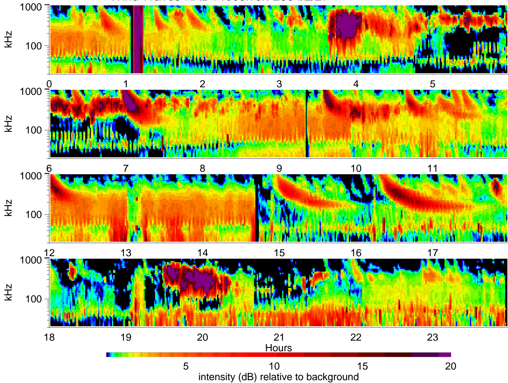
Wind Waves RAD1 receiver: 2004/2/27
