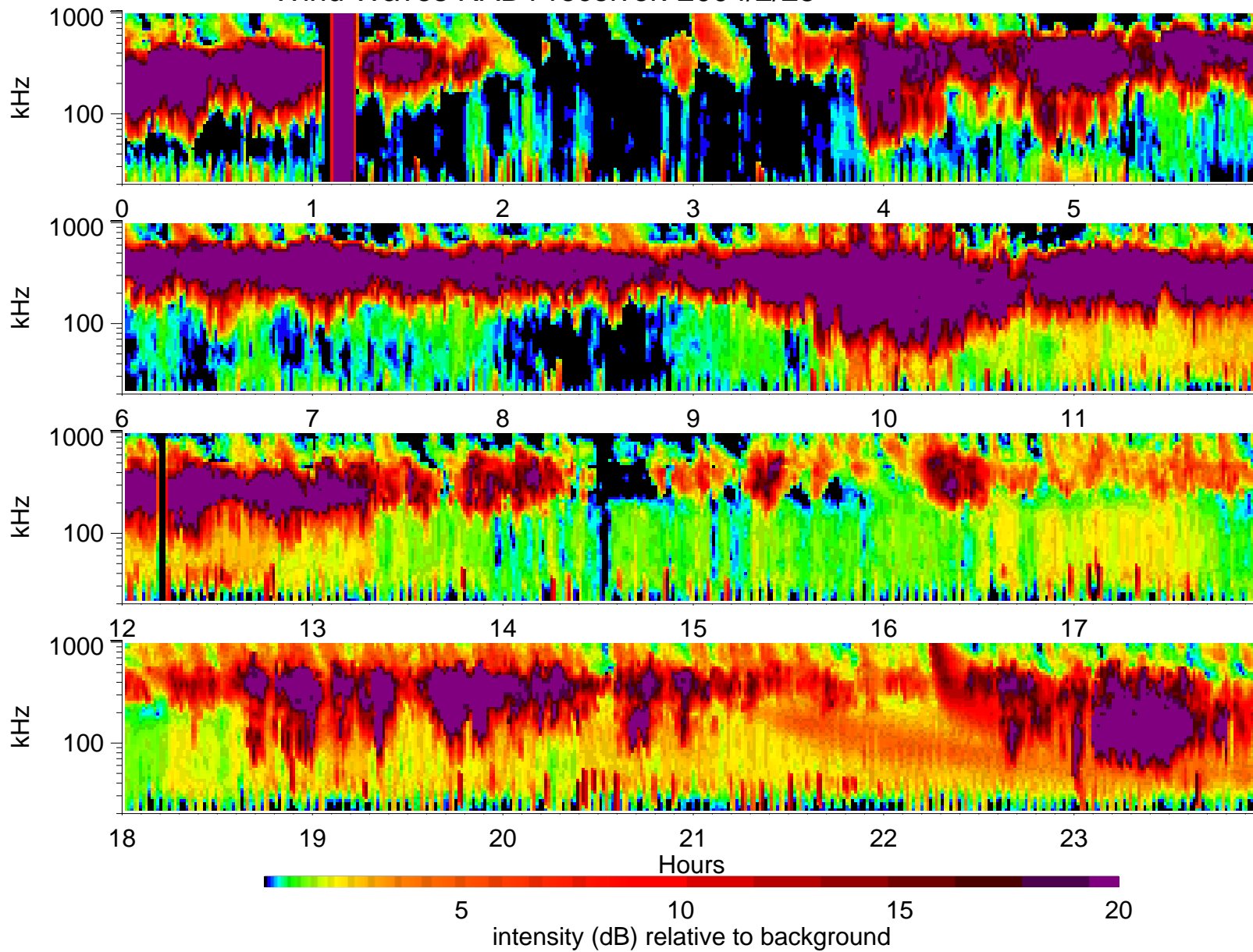
Wind Waves RAD1 receiver: 2004/2/25
