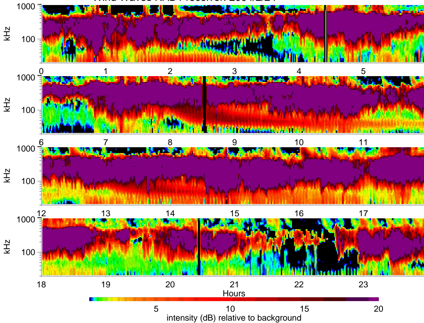
Wind Waves RAD1 receiver: 2004/2/24
