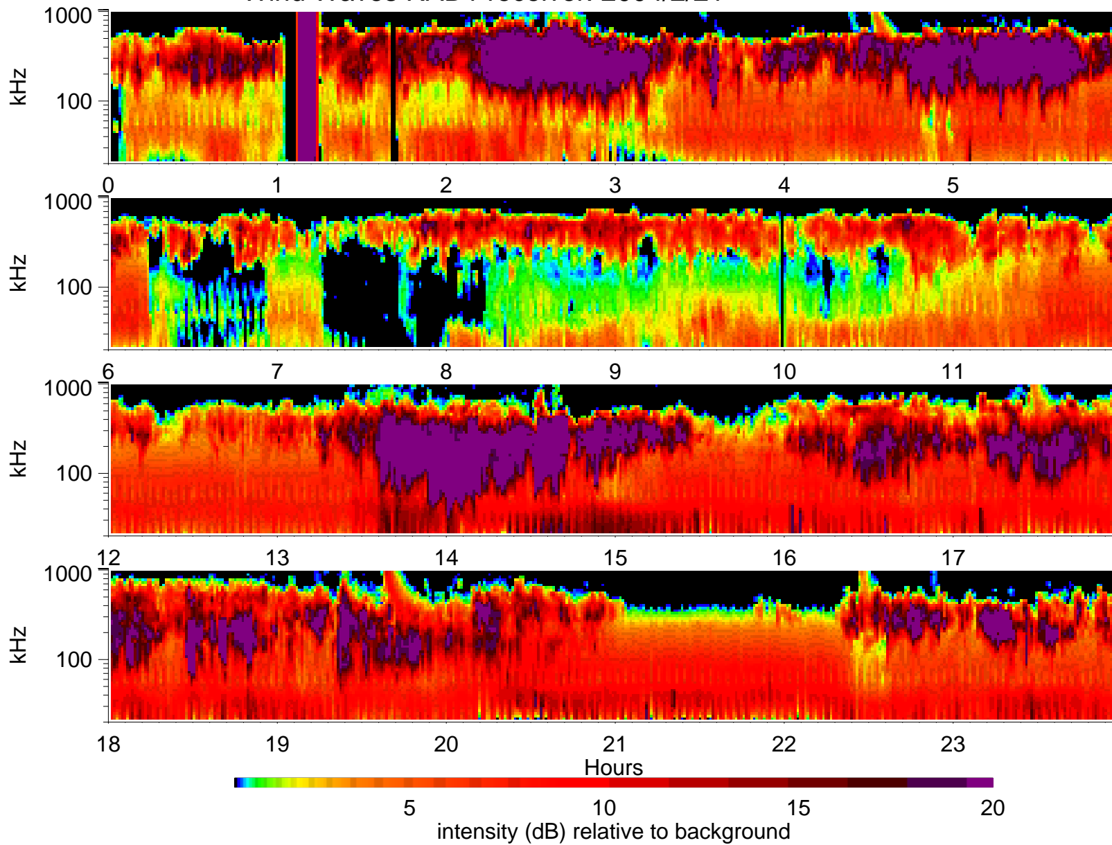
Wind Waves RAD1 receiver: 2004/2/21
