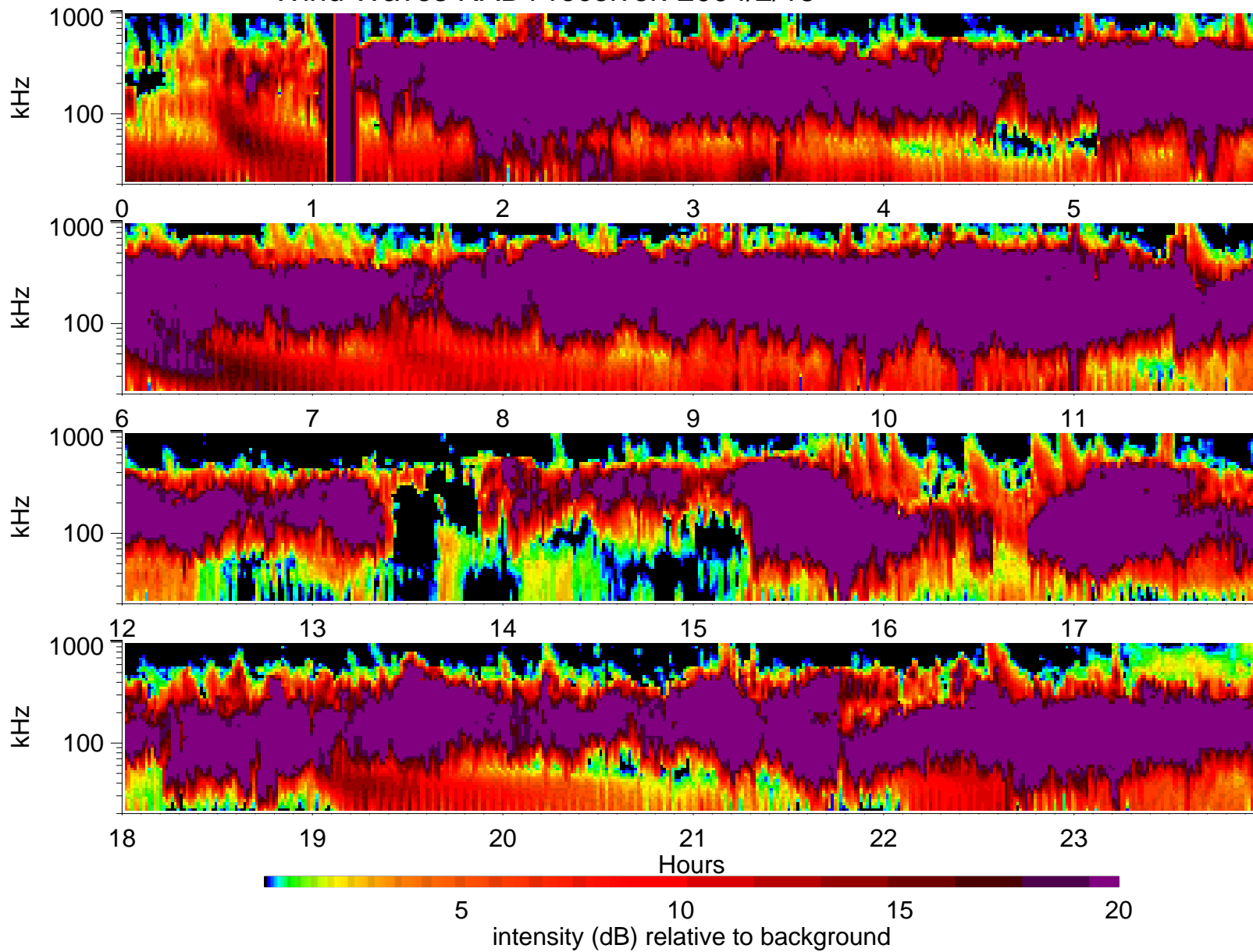
Wind Waves RAD1 receiver: 2004/2/15
