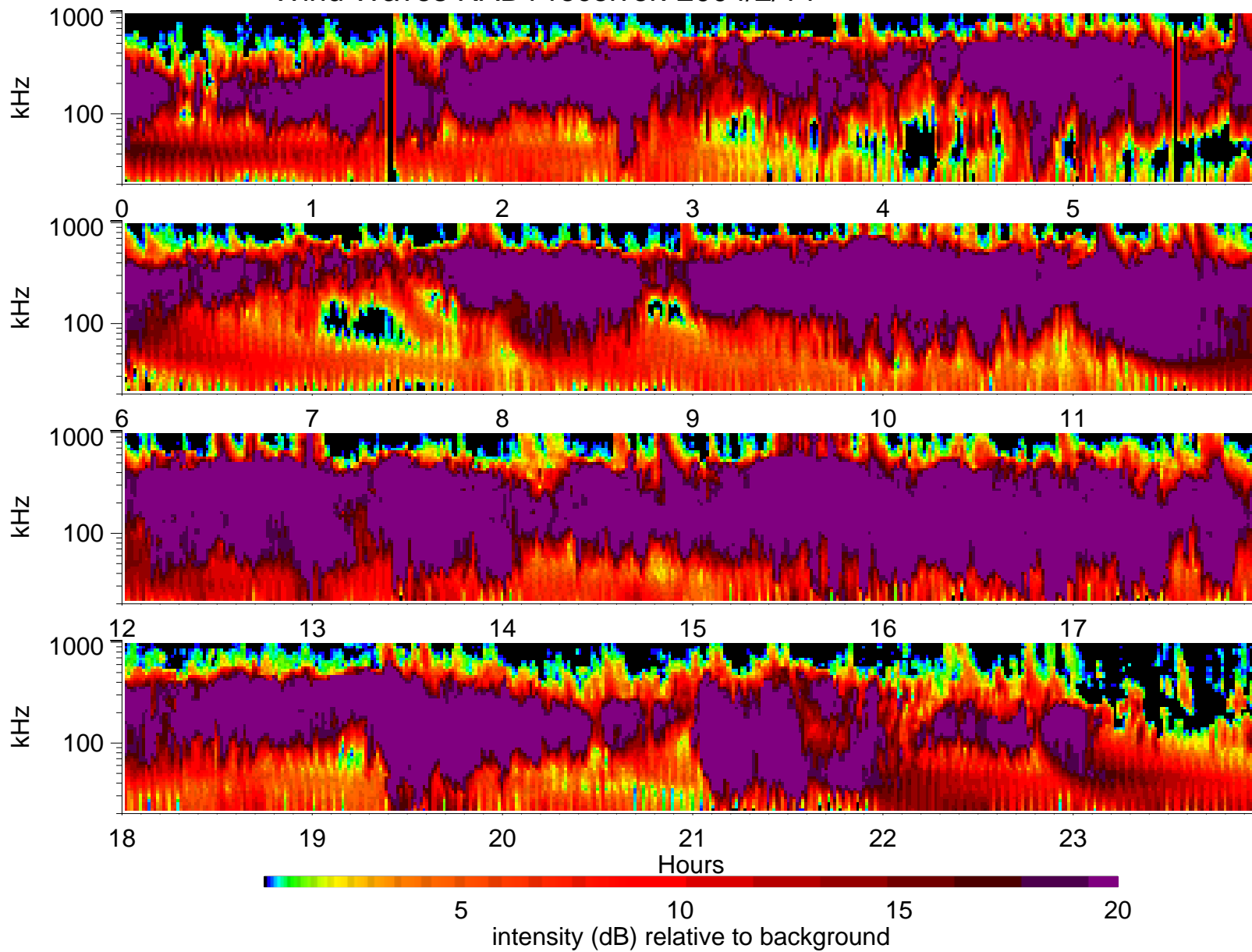
Wind Waves RAD1 receiver: 2004/2/14
