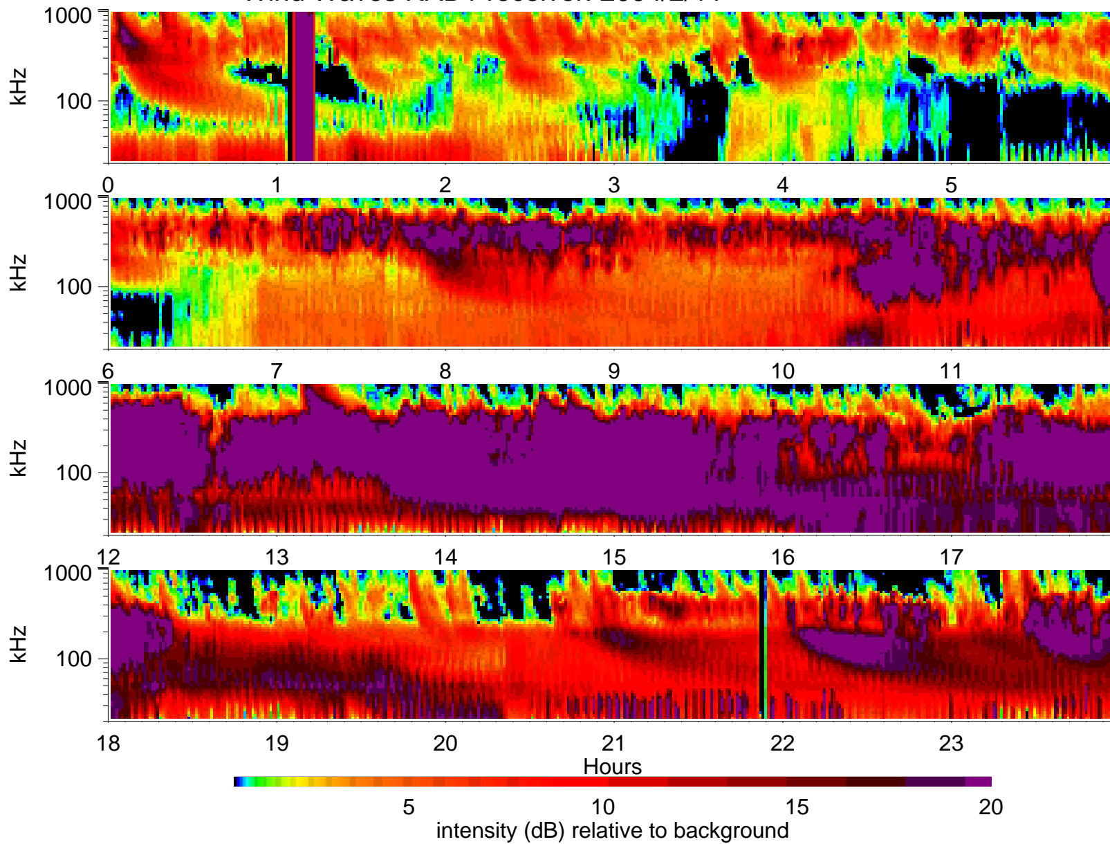
Wind Waves RAD1 receiver: 2004/2/11
