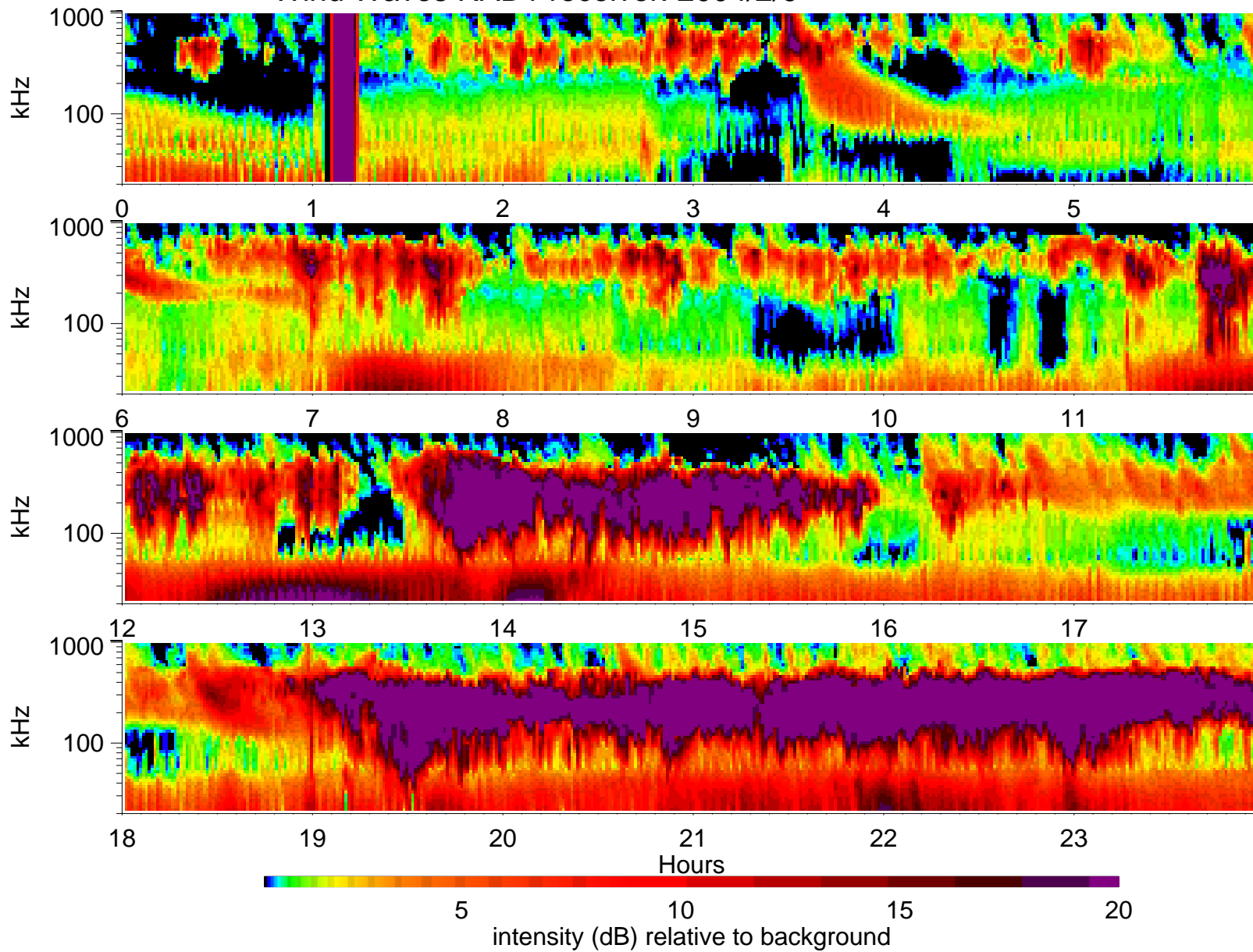
Wind Waves RAD1 receiver: 2004/2/9
