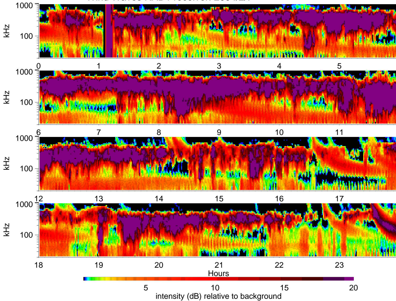
Wind Waves RAD1 receiver: 2004/2/7
