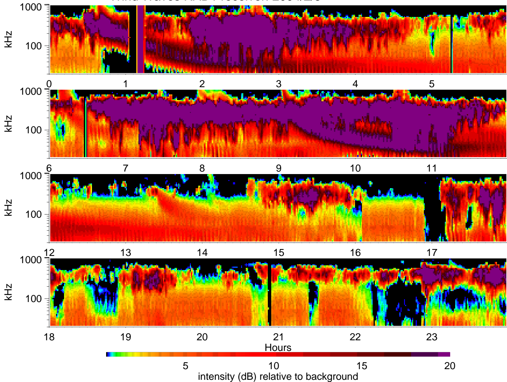
Wind Waves RAD1 receiver: 2004/2/5
