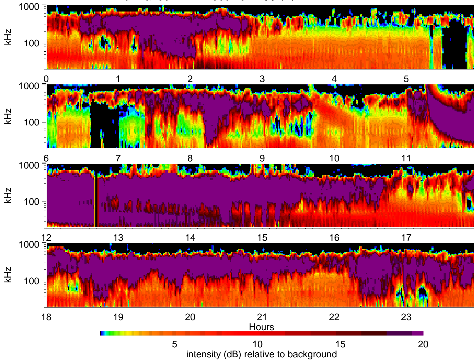
Wind Waves RAD1 receiver: 2004/2/4
