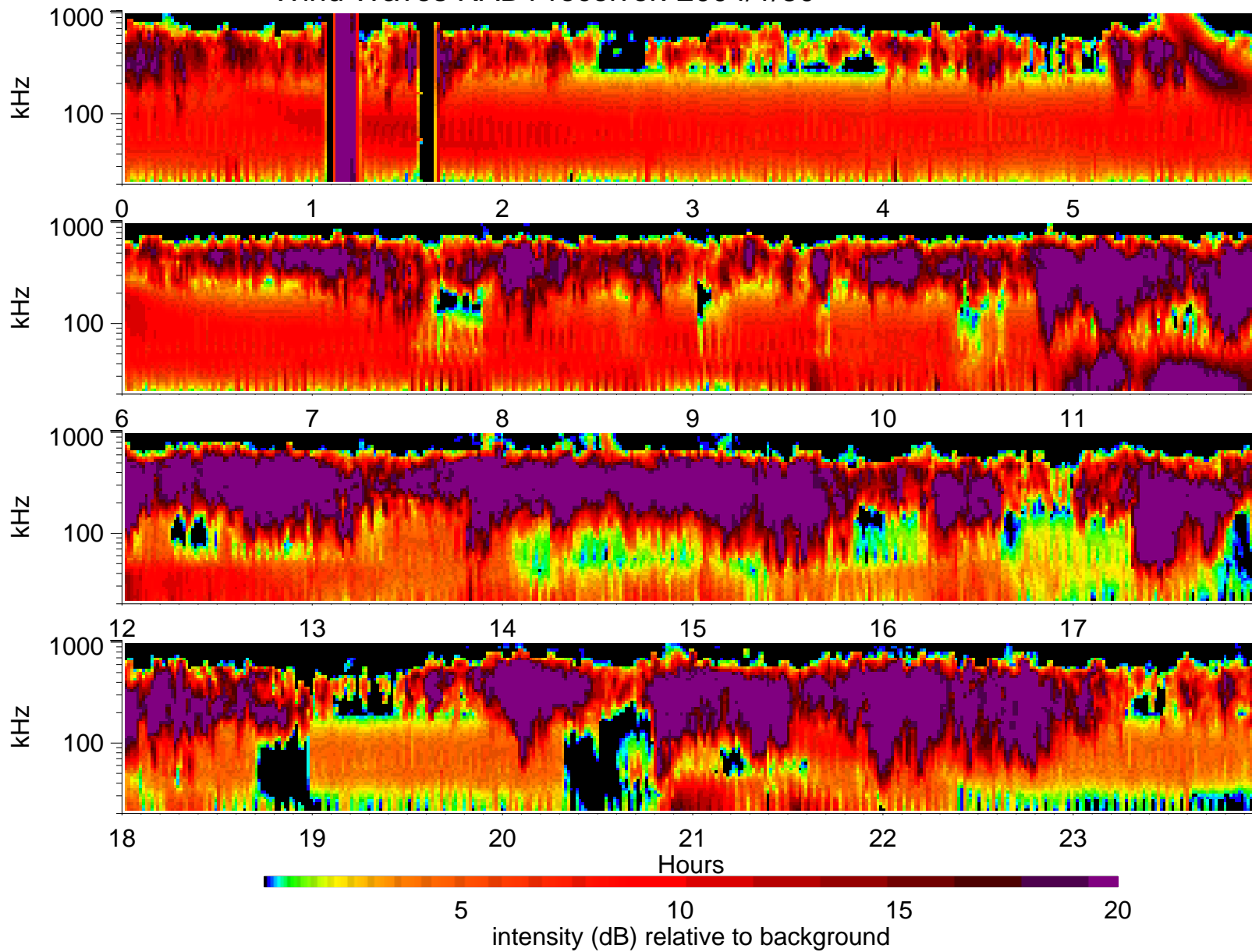
Wind Waves RAD1 receiver: 2004/1/30
