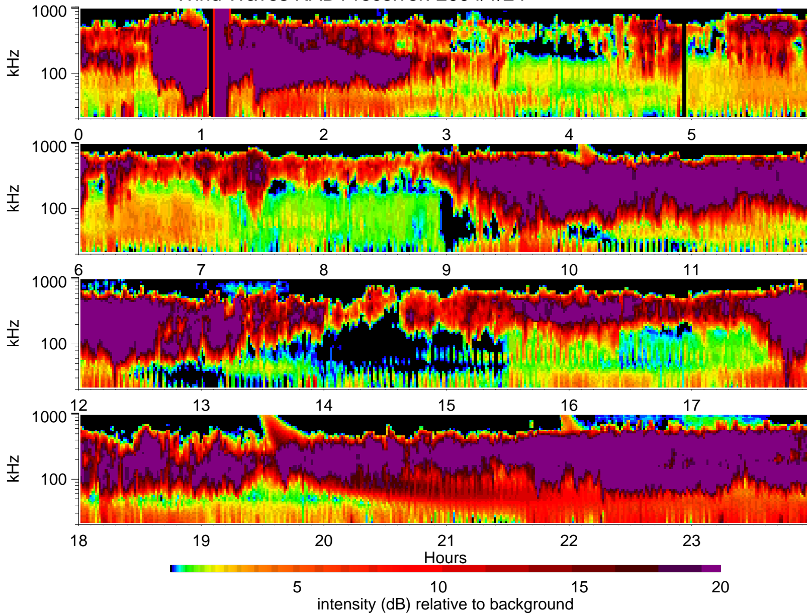
Wind Waves RAD1 receiver: 2004/1/24
