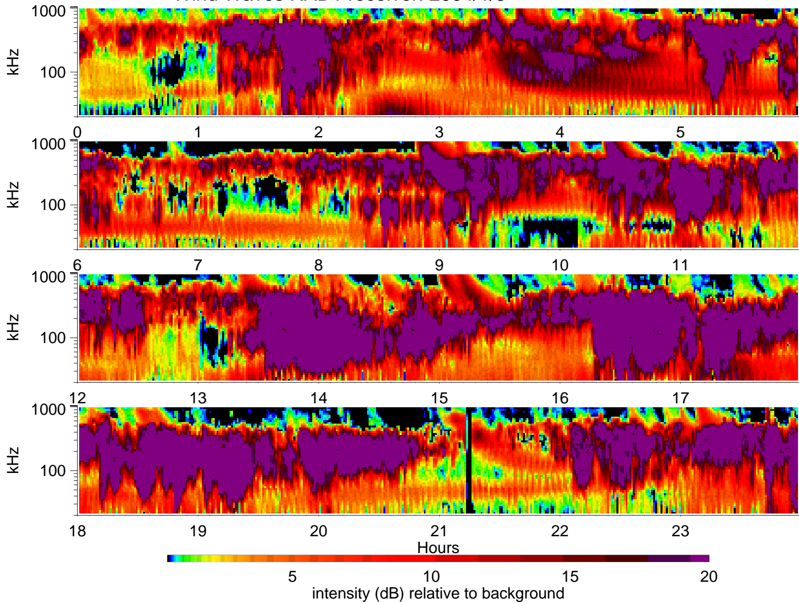
Wind Waves RAD1 receiver: 2004/1/5
