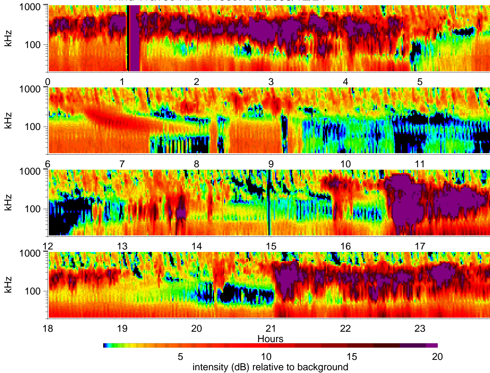
Wind Waves RAD1 receiver: 2003/12/24
