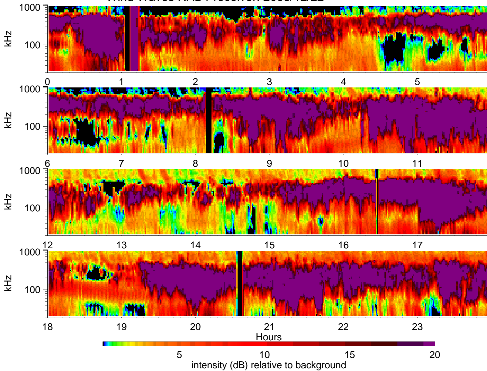
Wind Waves RAD1 receiver: 2003/12/22
