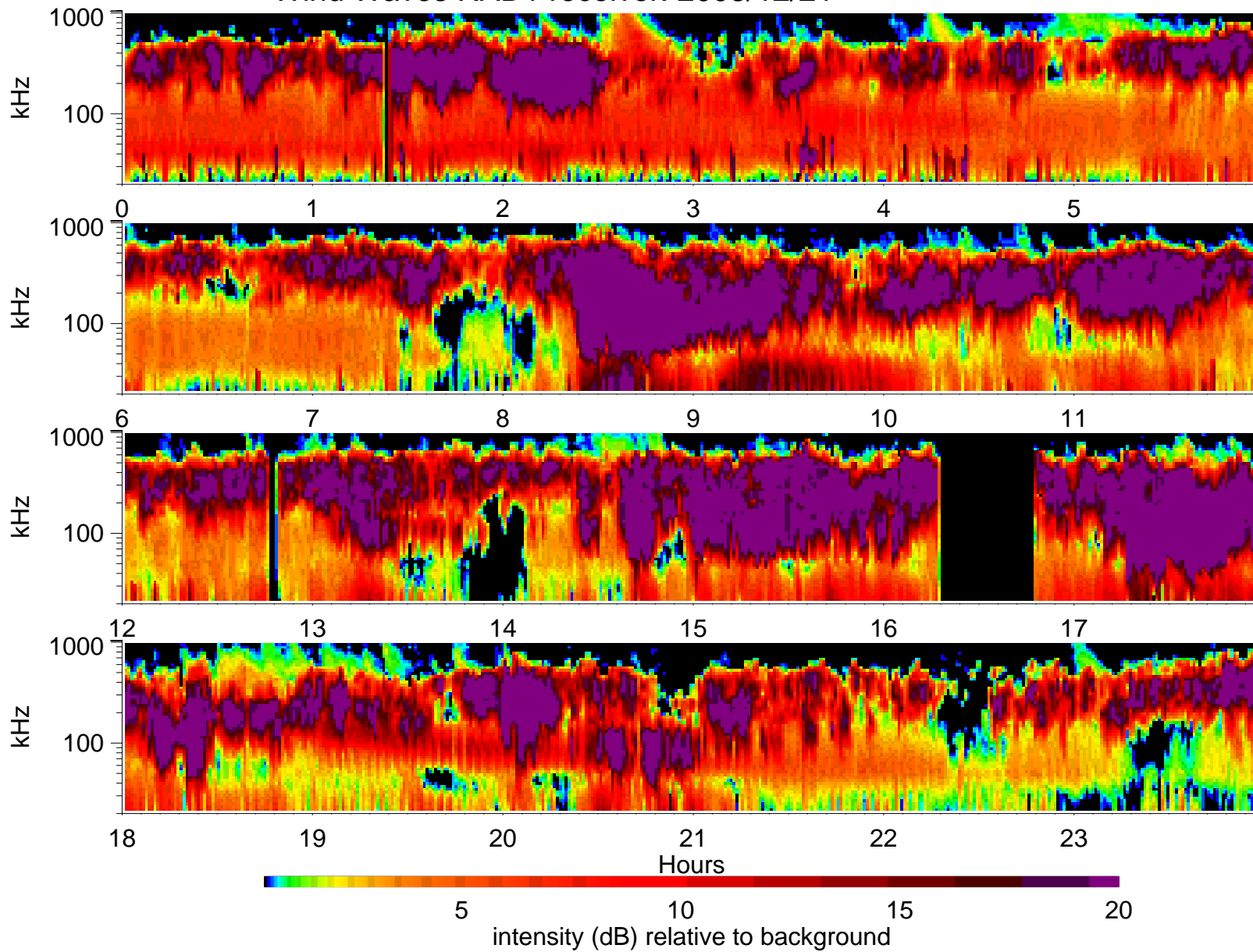
Wind Waves RAD1 receiver: 2003/12/21
