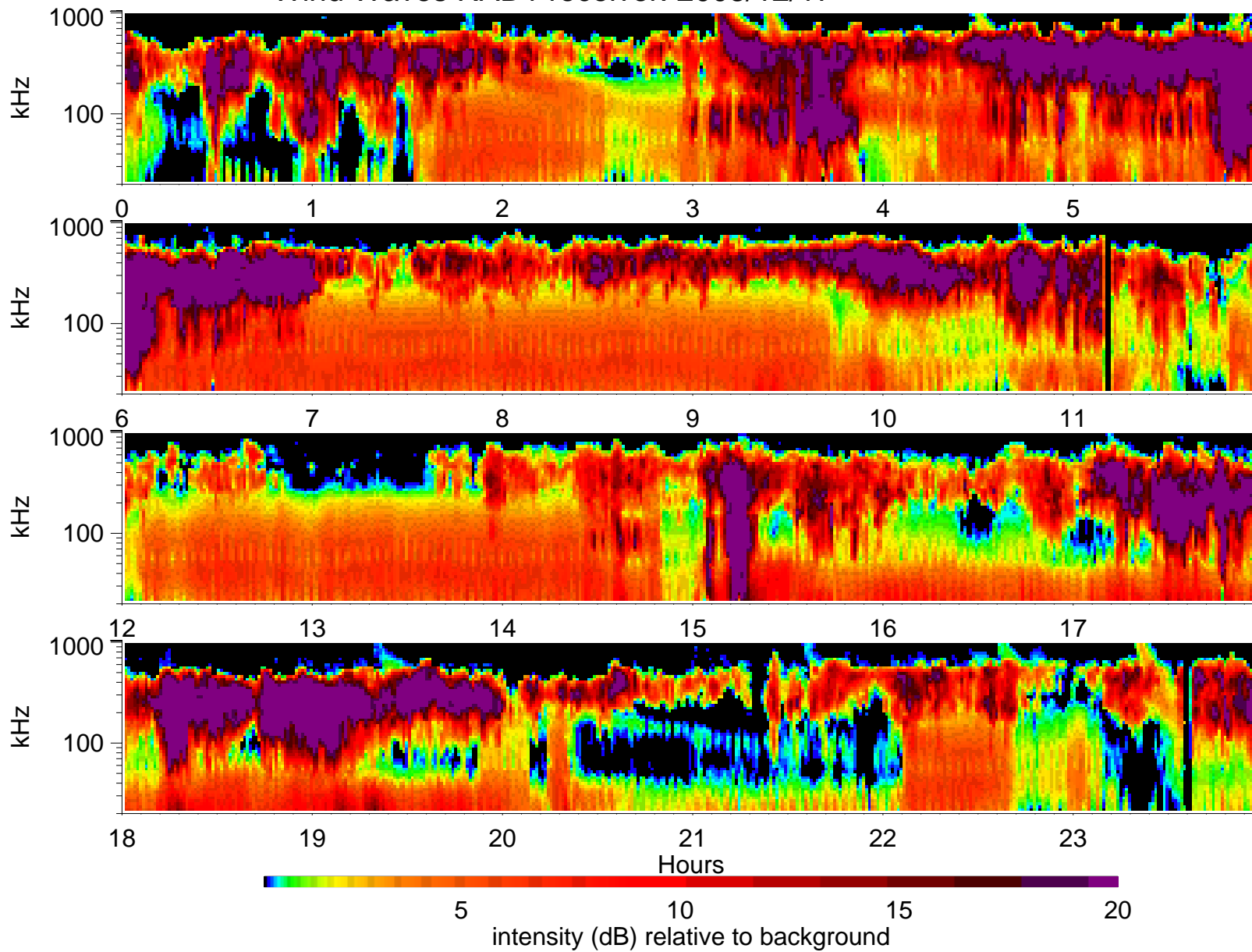
Wind Waves RAD1 receiver: 2003/12/17
