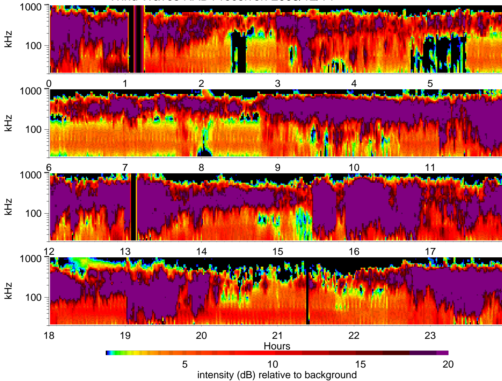
Wind Waves RAD1 receiver: 2003/12/14
