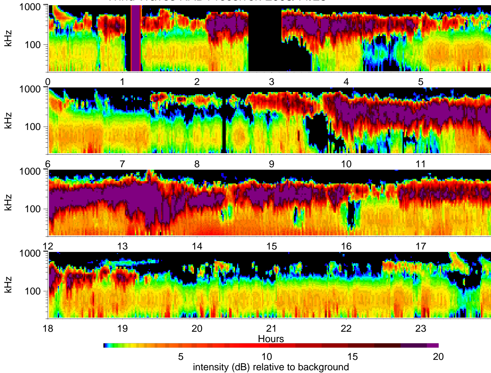
Wind Waves RAD1 receiver: 2003/11/28
