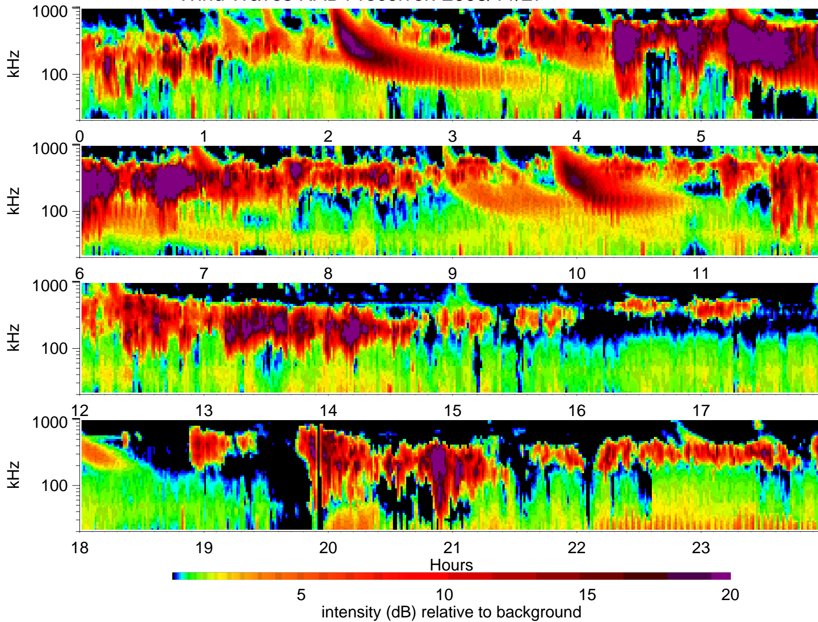
Wind Waves RAD1 receiver: 2003/11/27
