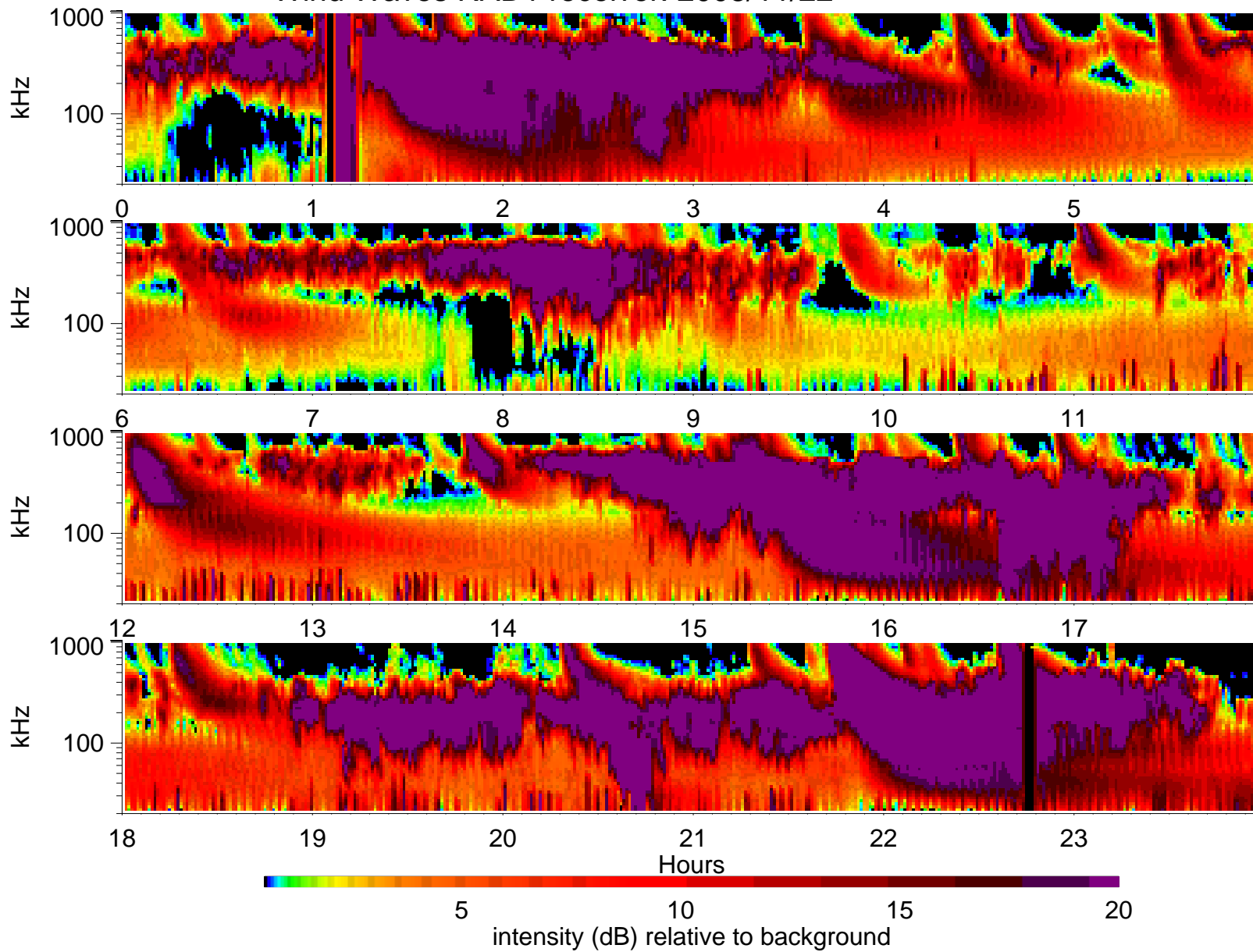
Wind Waves RAD1 receiver: 2003/11/22
