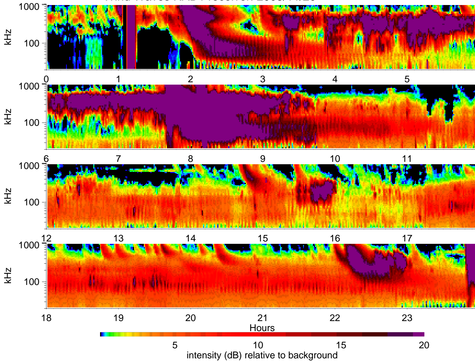
Wind Waves RAD1 receiver: 2003/11/20
