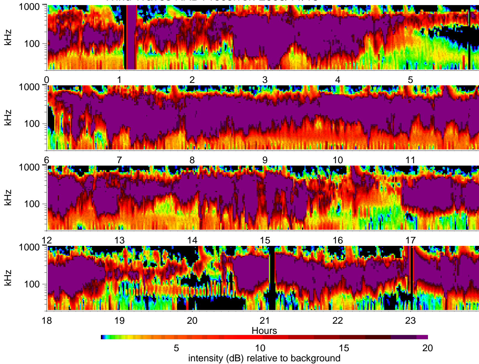
Wind Waves RAD1 receiver: 2003/11/16
