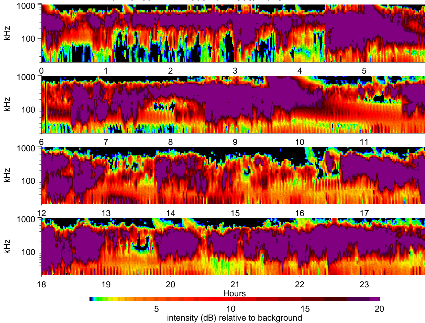
Wind Waves RAD1 receiver: 2003/11/13
