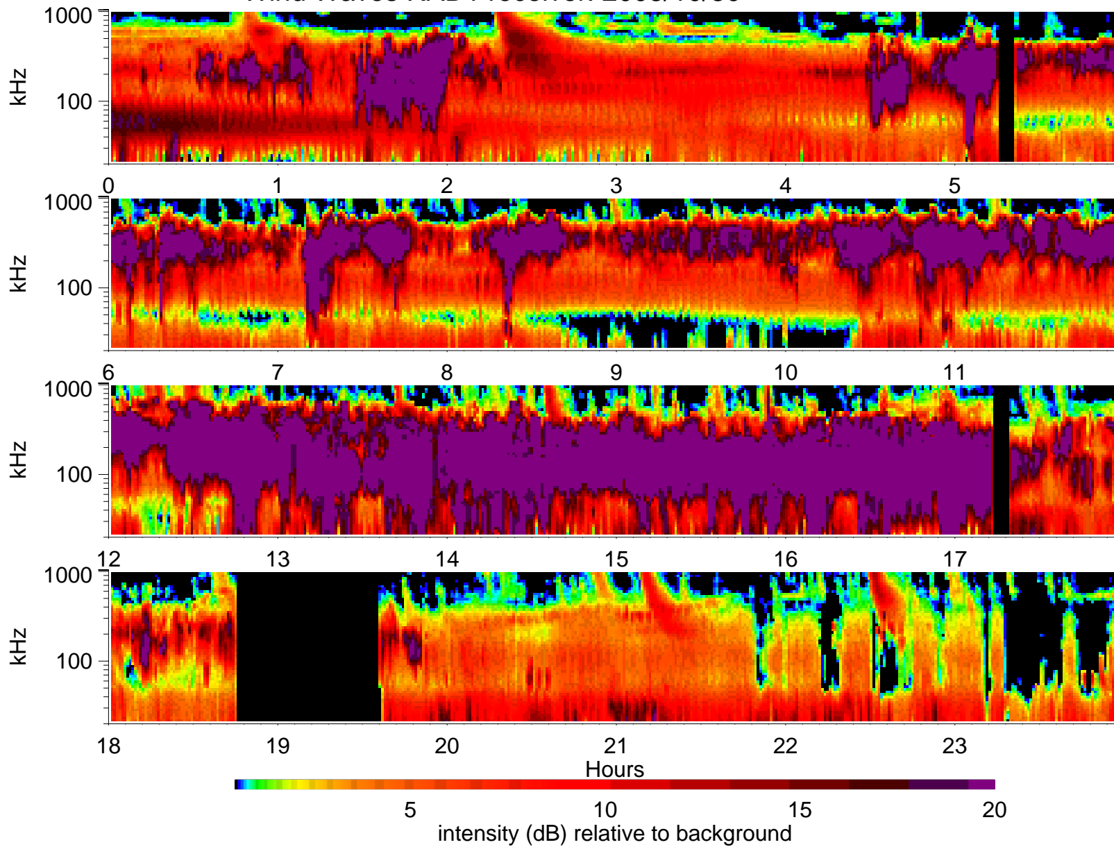
Wind Waves RAD1 receiver: 2003/10/30
