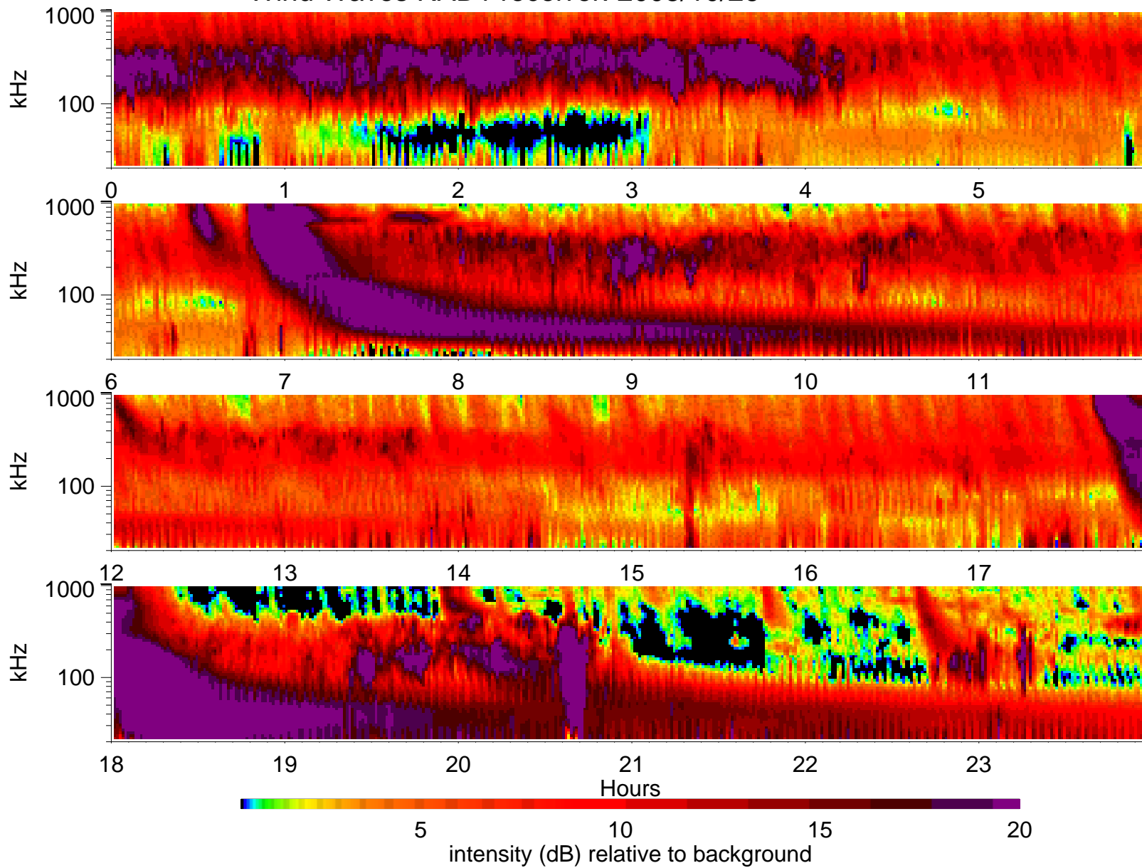
Wind Waves RAD1 receiver: 2003/10/26
