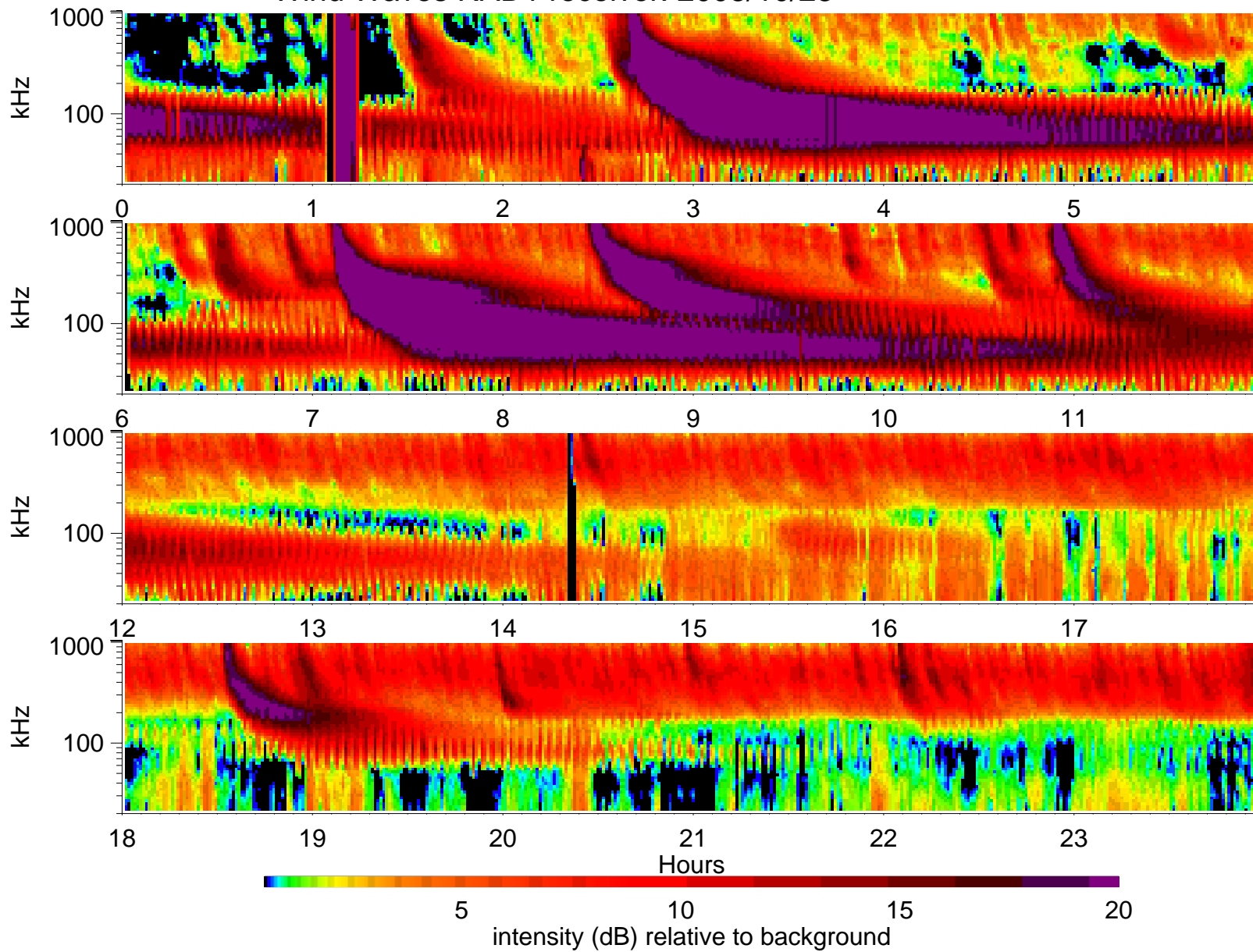
Wind Waves RAD1 receiver: 2003/10/23
