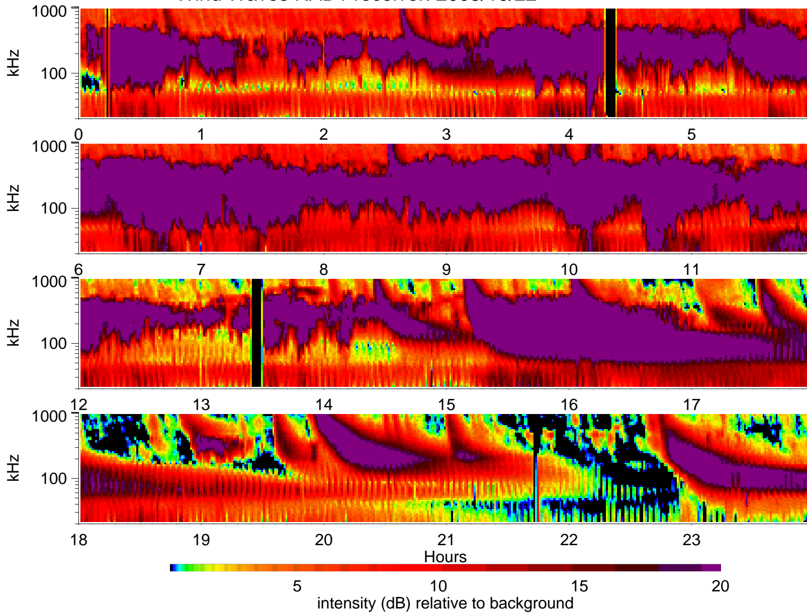
Wind Waves RAD1 receiver: 2003/10/22
