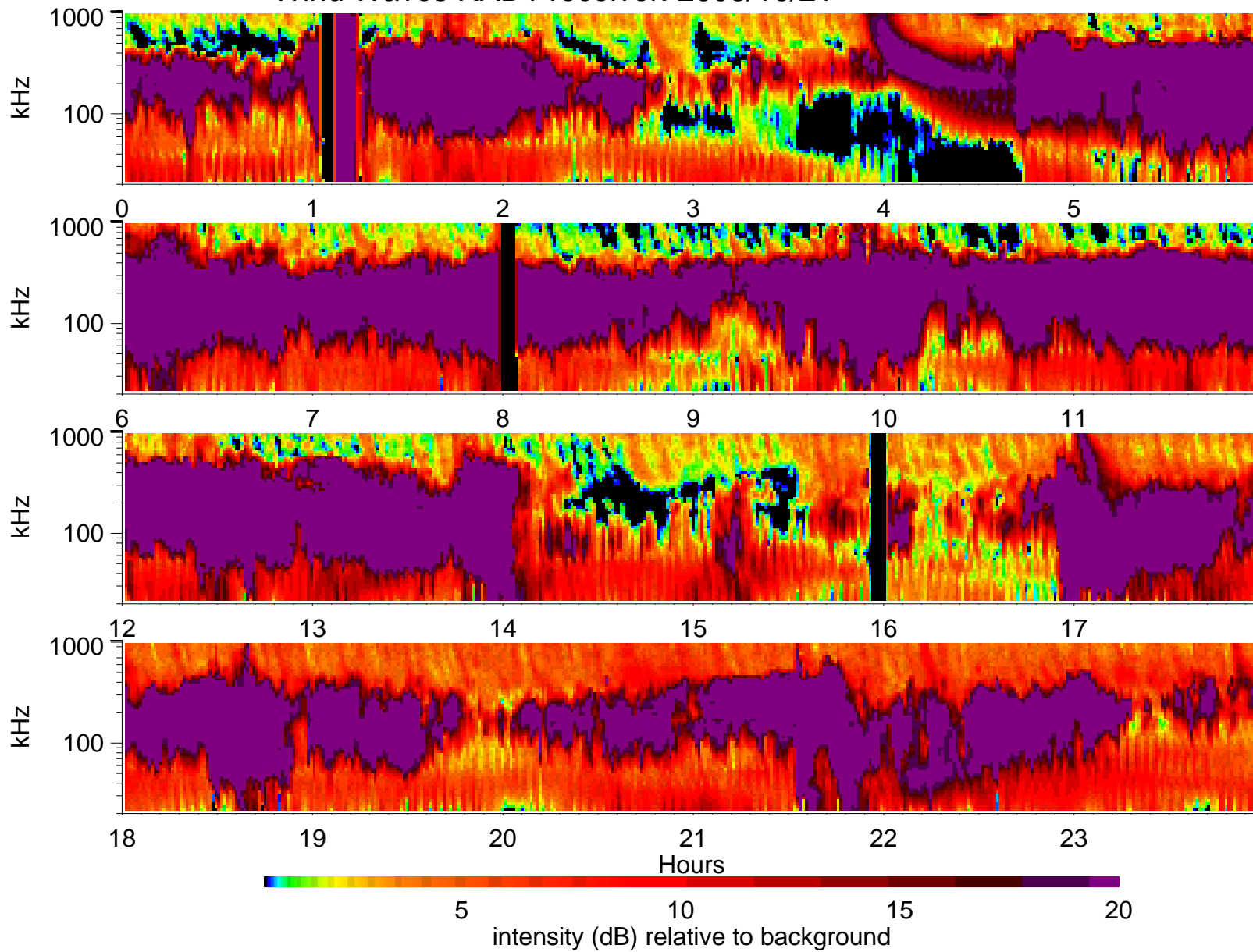
Wind Waves RAD1 receiver: 2003/10/21
