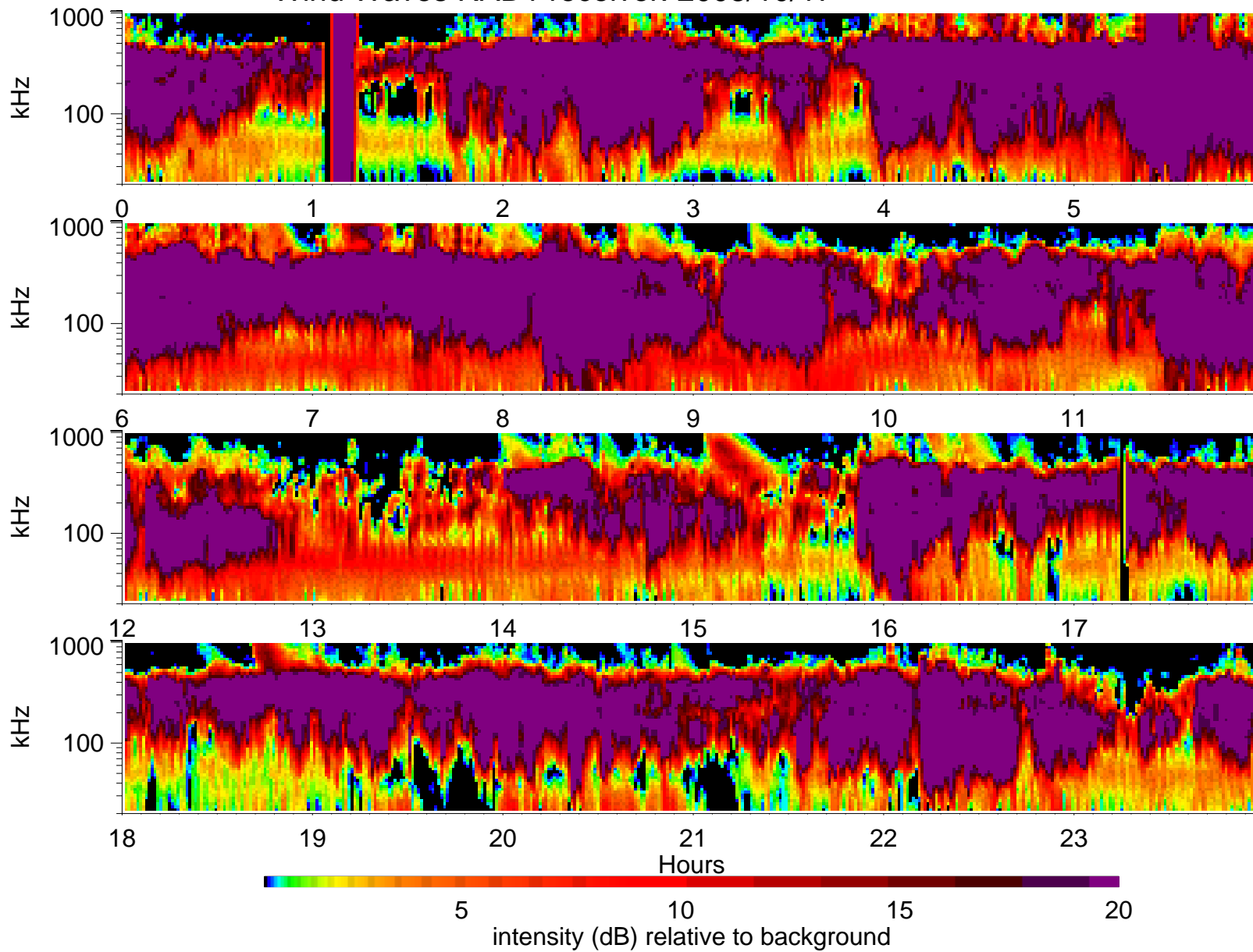
Wind Waves RAD1 receiver: 2003/10/17
