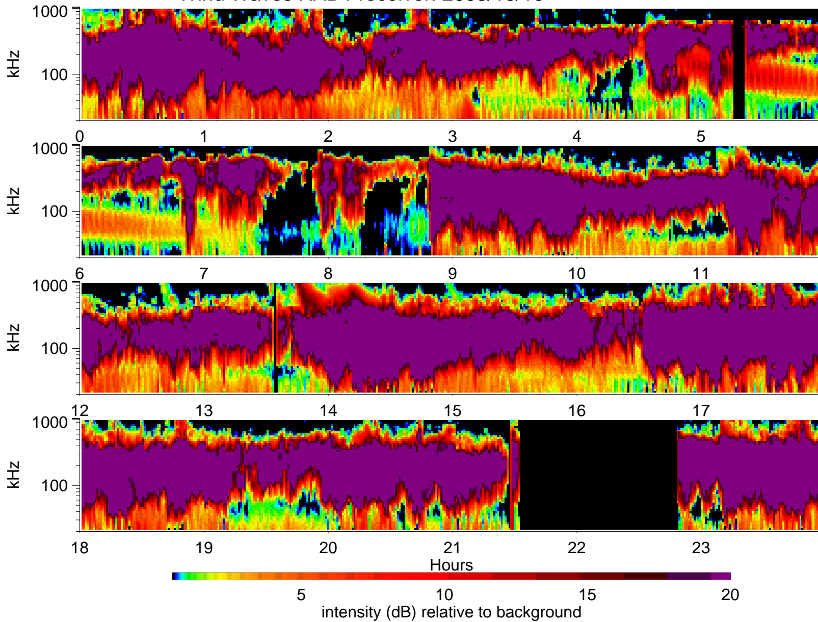
Wind Waves RAD1 receiver: 2003/10/16
