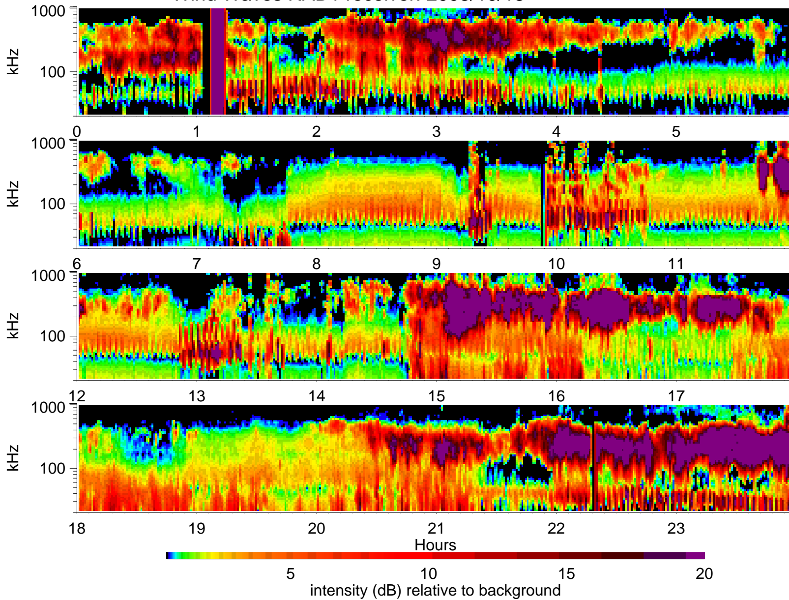
Wind Waves RAD1 receiver: 2003/10/13
