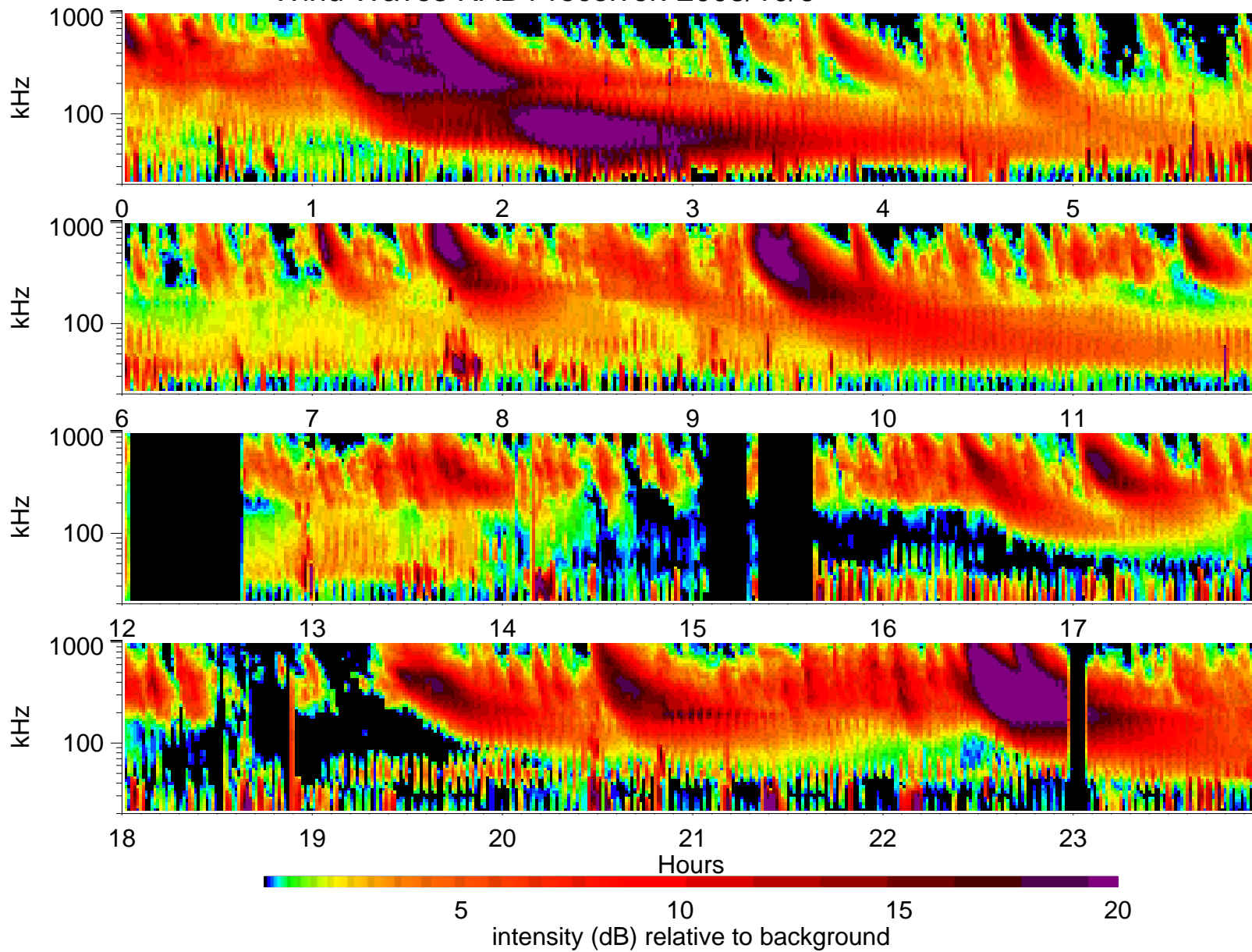
Wind Waves RAD1 receiver: 2003/10/6
