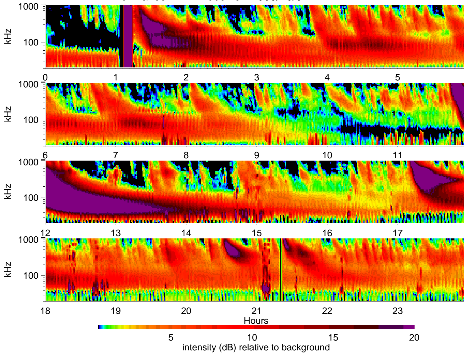
Wind Waves RAD1 receiver: 2003/10/5
