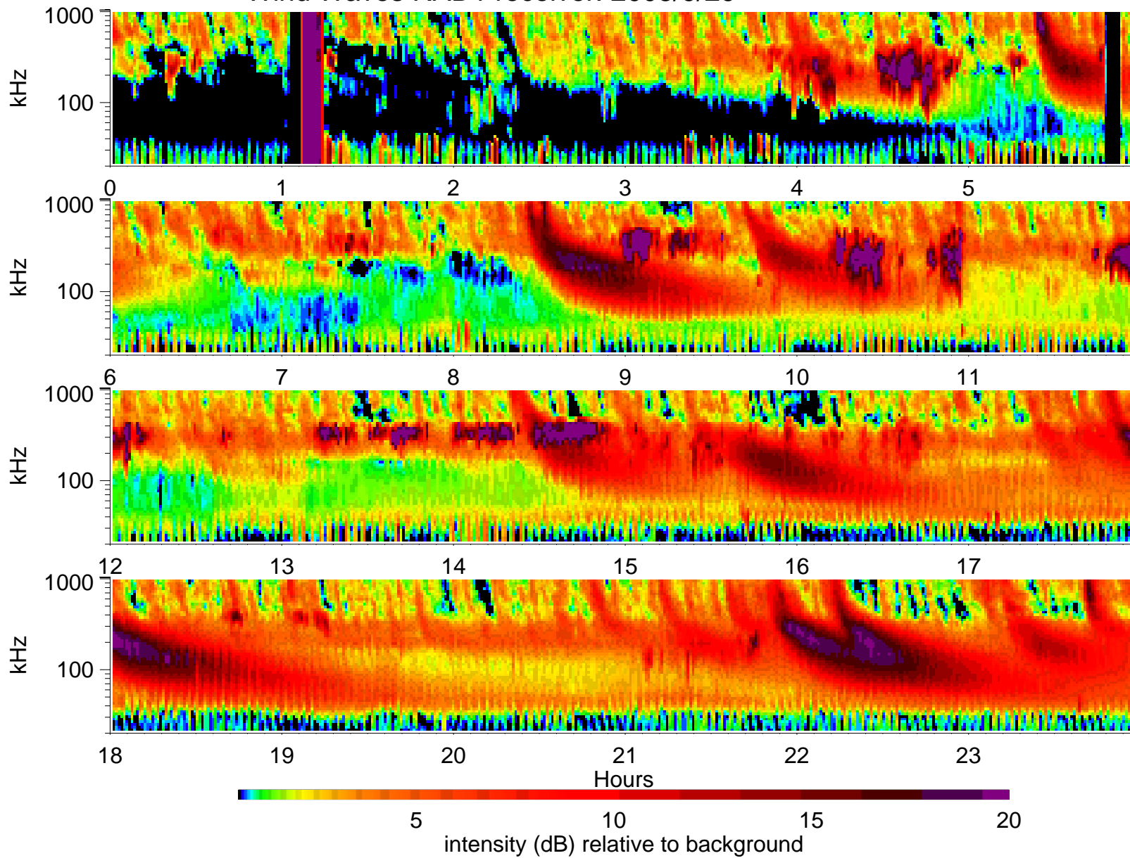
Wind Waves RAD1 receiver: 2003/9/29
