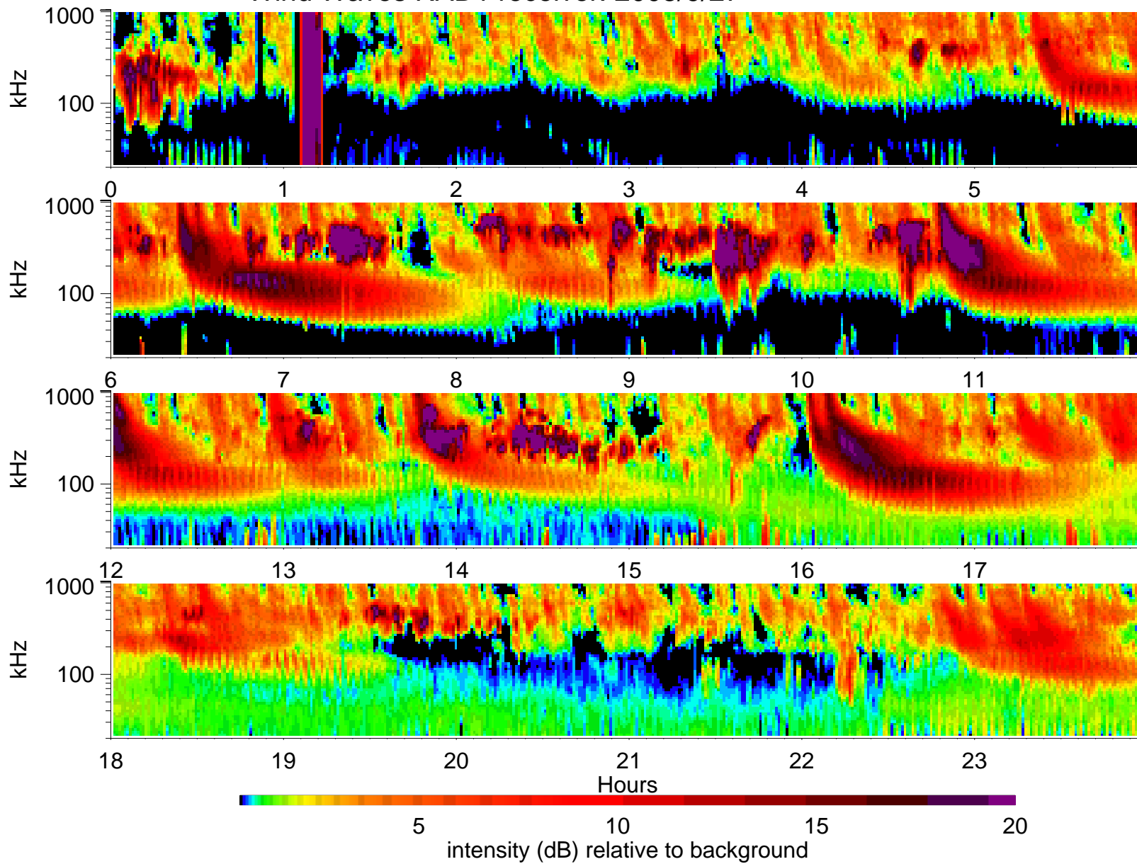
Wind Waves RAD1 receiver: 2003/9/27
