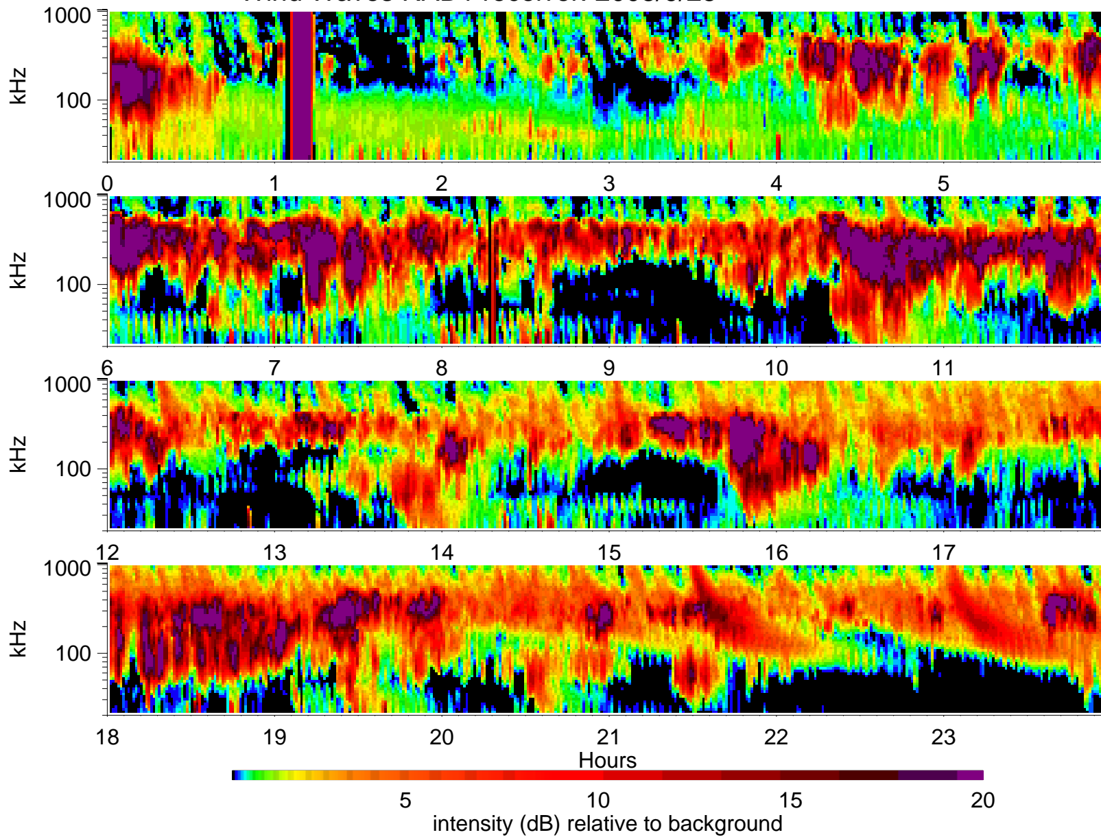
Wind Waves RAD1 receiver: 2003/9/25
