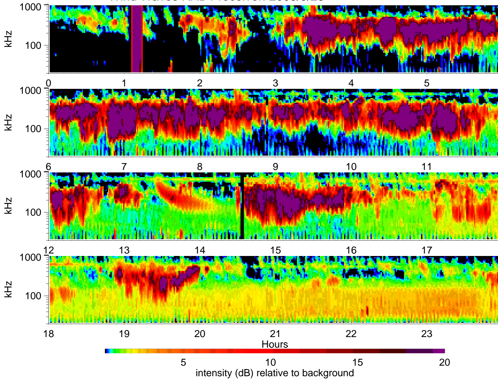
Wind Waves RAD1 receiver: 2003/9/23
