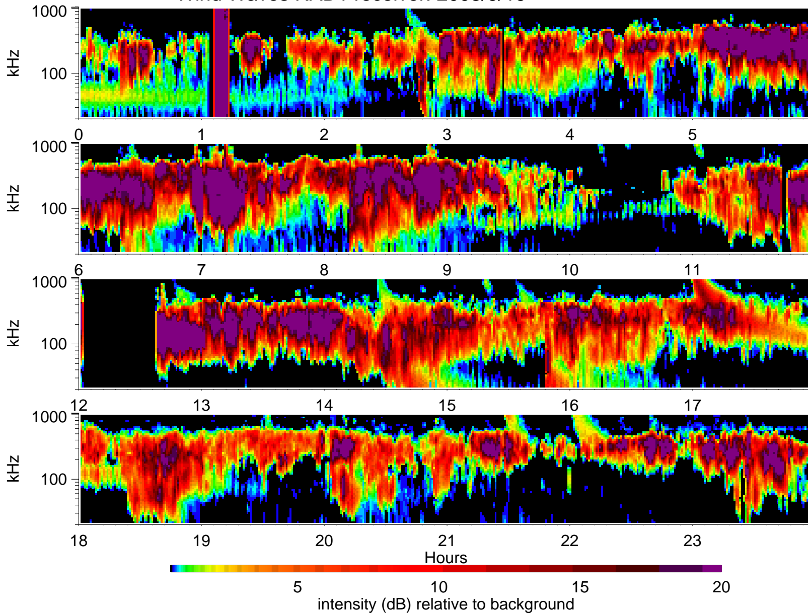
Wind Waves RAD1 receiver: 2003/9/19
