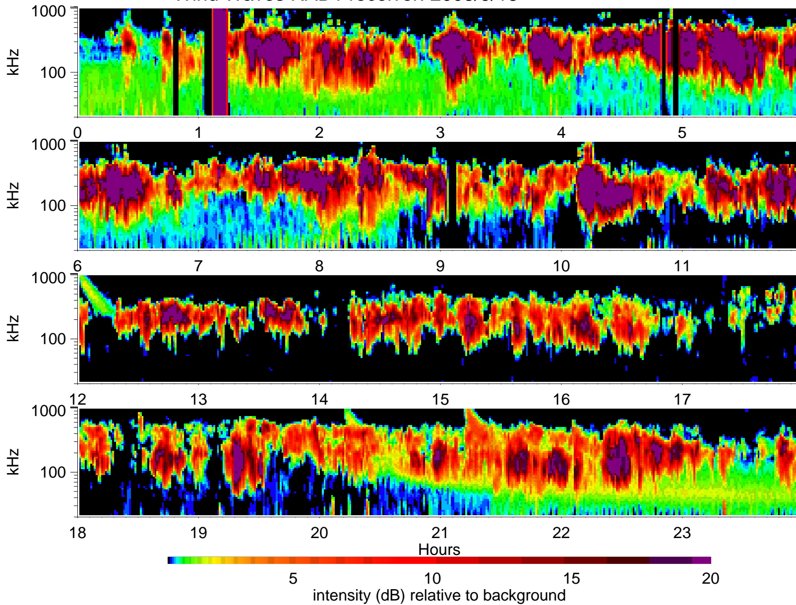
Wind Waves RAD1 receiver: 2003/9/13
