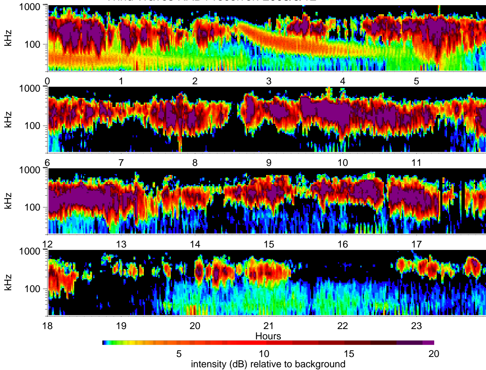
Wind Waves RAD1 receiver: 2003/9/12
